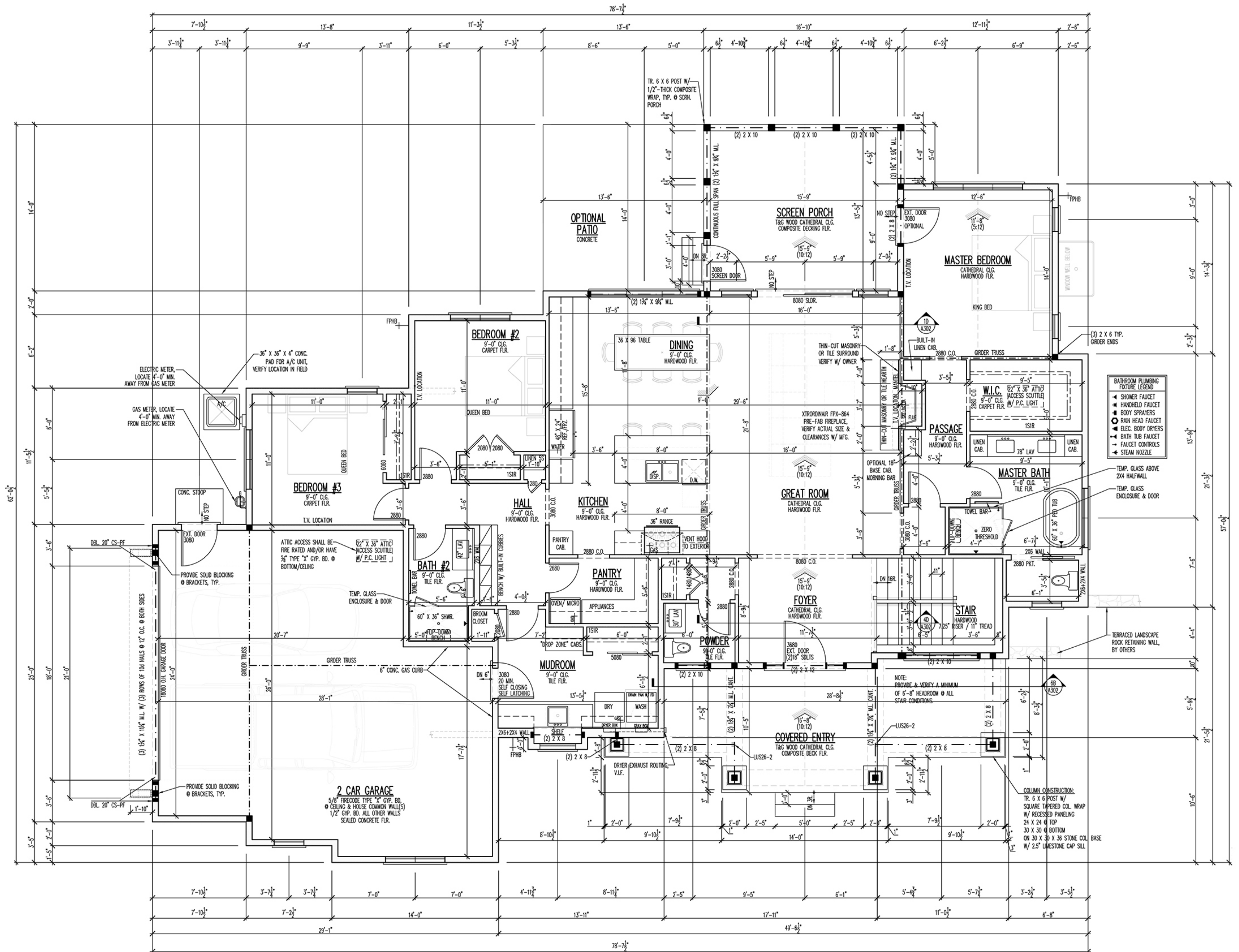
1E A101 FIRST FLOOR PLAN
