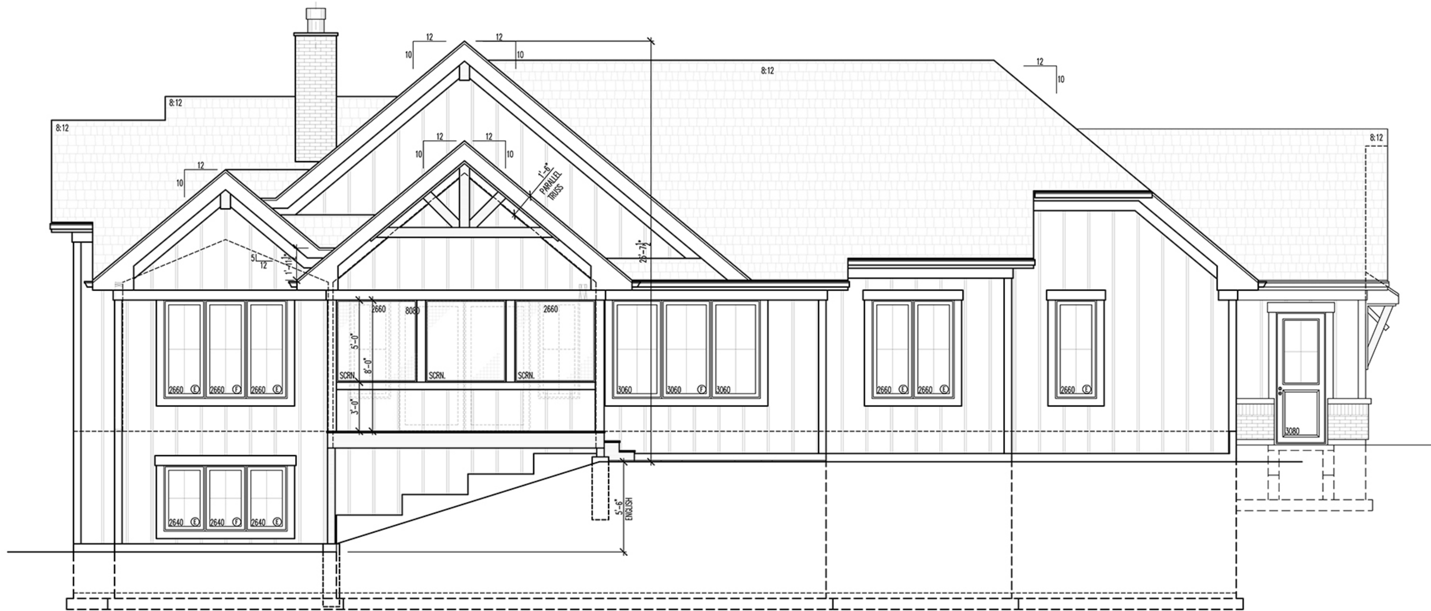
1C A200 REAR ELEVATION
